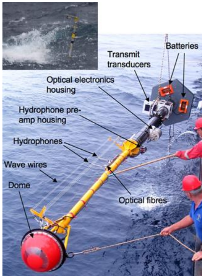
Figure 6. An example of the spar buoy capacitance wire system deployed in the Southern ocean (top left insert) and North Atlantic (main figure).
