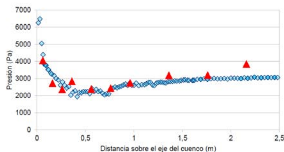
Figure 14 Pressure distribution on the central axis of the stilling basin. In abscissa the distance from the toe of the dam.
