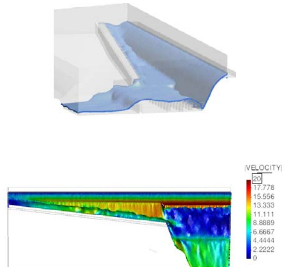
Figure 16 Geometry of the emergency spillway with highly convergent chutes (above) and velocity contour fill of the overtopping simulation (below).
