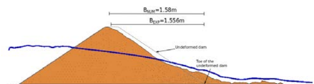
Figure 3 Evolution of the free surface/seepage line (in blue) and of the deformation of the downstream shoulder in a homogeneous dam for an incoming discharge of 90.68L/s. Source [Salazar et al. 2016].
