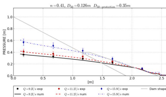
Figure 2 Numerical and experimental comparison of pressure heads distribution at the bottom of the multilayer dam. Three different incoming discharge have been considered: 9.2l/s (continuous line), 11.2l/s (dotted line), 15.9l/s (pointed line). Source [Larese 2015a].
