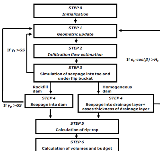
Figure 9 Flowchart of the algorithm of the design procedure proposed. GS: maximum saturation rate input; H_t : height of toe; y_t : maximum seepage level under the flip bucket struc-
