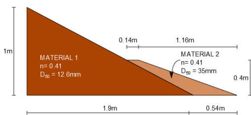
Figure 1 Geometry of the dam with protection on the downstream toe and characteristics of the materials.
