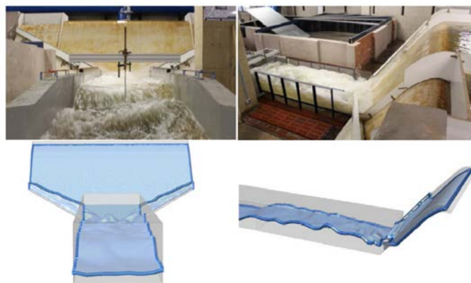
Figure 13 Numerical (above) and experimental (below) tests on a symmetric configuration of the converging chutes with slope 2:1.
