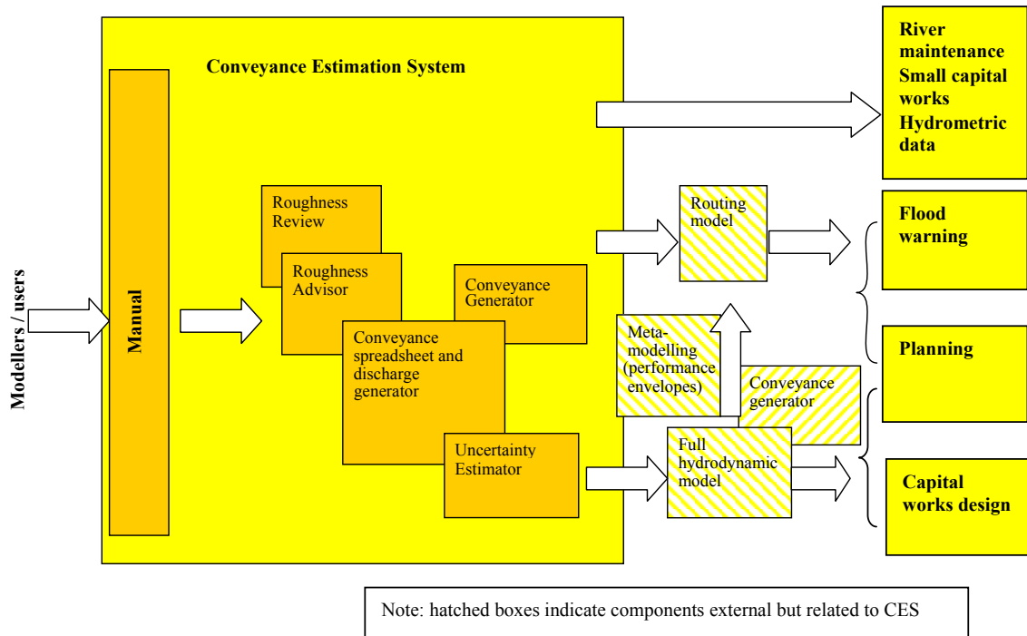
Figure 3 Components of the Conveyance Estimation System
